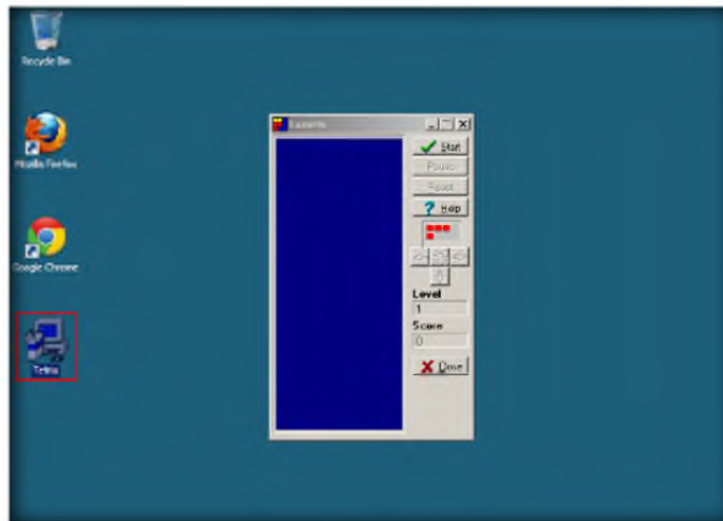
FIGURE 3.7: Lazaris game
