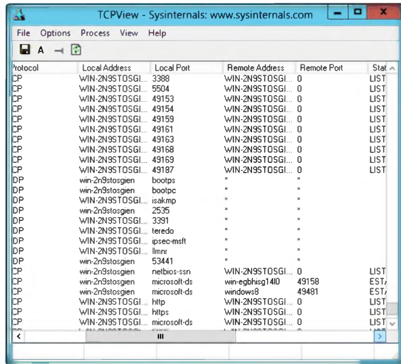
FIGURE 8.3: Tcpview analyzing ports
