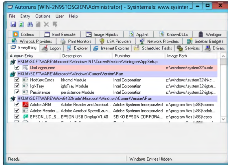
FIGURE 8.5: Autoruns Main Window
