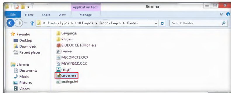
FIGURE 9.5: Bidox services
