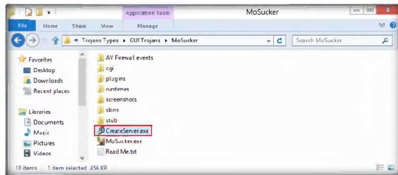
FIGURE 10.1: Install createServer.exe
