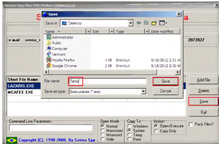
FIGURE 3.6: Trojan created
