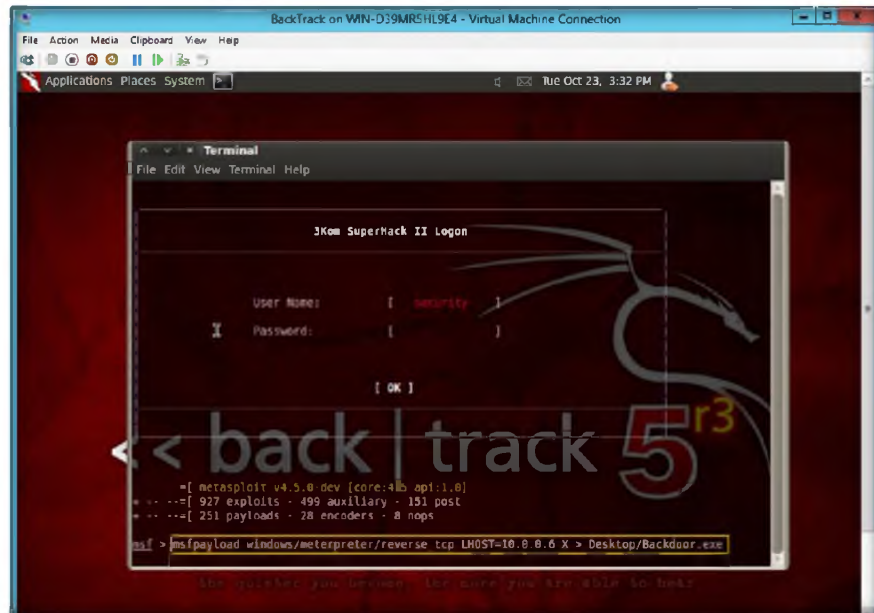
FIGURE 11.2: Creating Backdoor.exe
