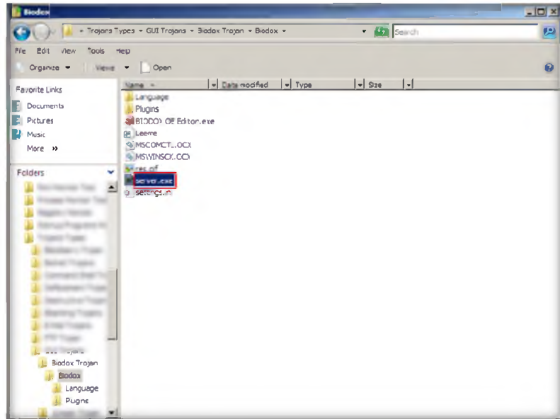
FIGURE 9.6: Biodox server.exe
