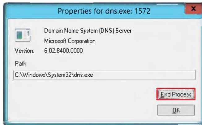
FIGURE 8.4: Killing Processes
