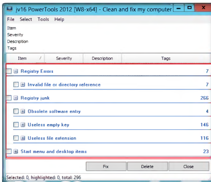
FIGURE 8.24: jv16 Clean and fix my computer Items details.
