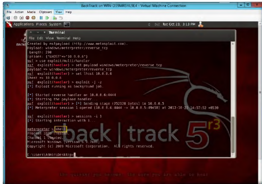
FIGURE 11.18: Type the shell command
