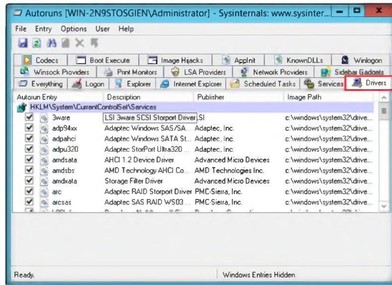
FIGURE 8.12: Autoruns Drivers list.
