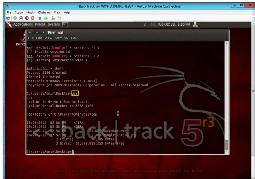
FIGURE 11.19: check the directories of windows 7
