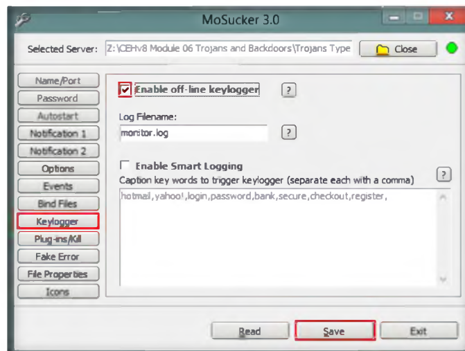
FIGURE 10.8: Enable the keylogger
