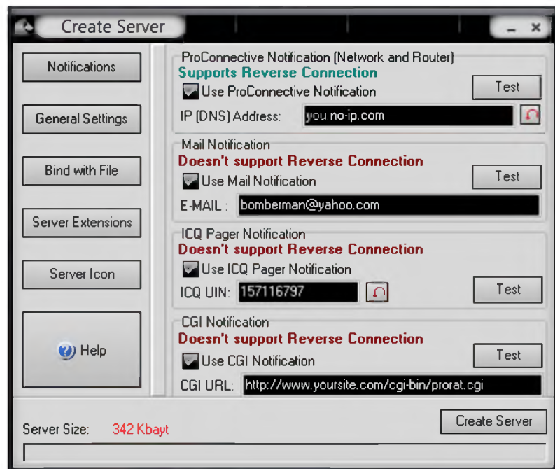
FIGURE 1.2: ProRat Create Server Window
