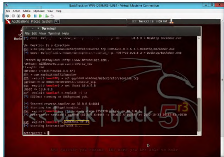
FIGURE 11.17: creating the session
