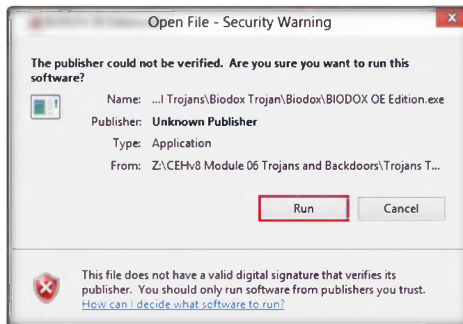
FIGURE 9.2: Windows 8-Security Warning
