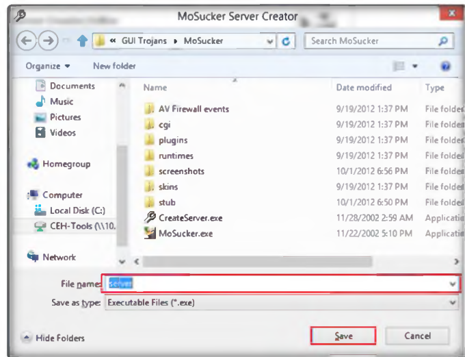
FIGURE 10.4: Save Server.exe
