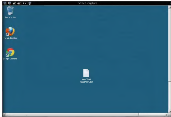
FIGURE 9.11: screen capture
