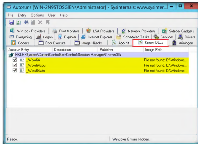
FIGURE 8.13: Autoruns Known DLL's list.
