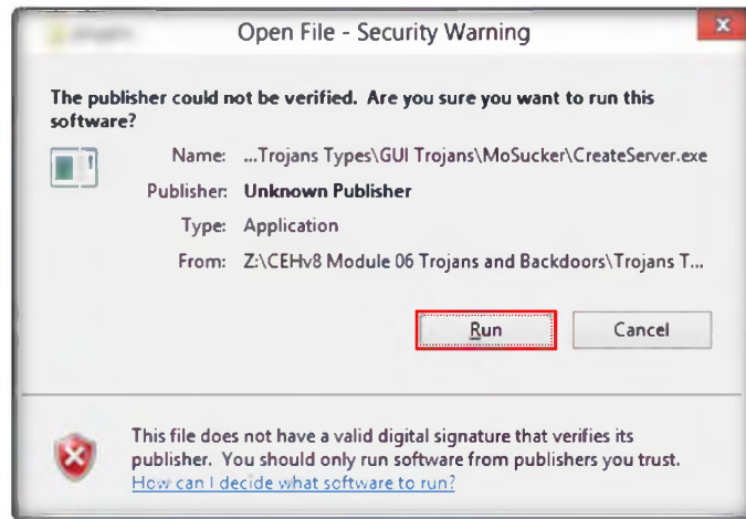
FIGURE 10.2: Install createServer.exe
