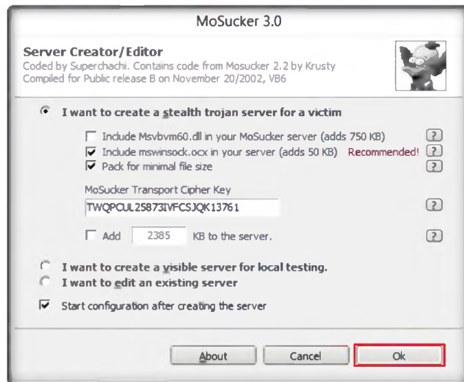
FIGURE 10.3: Install createServer.exe
