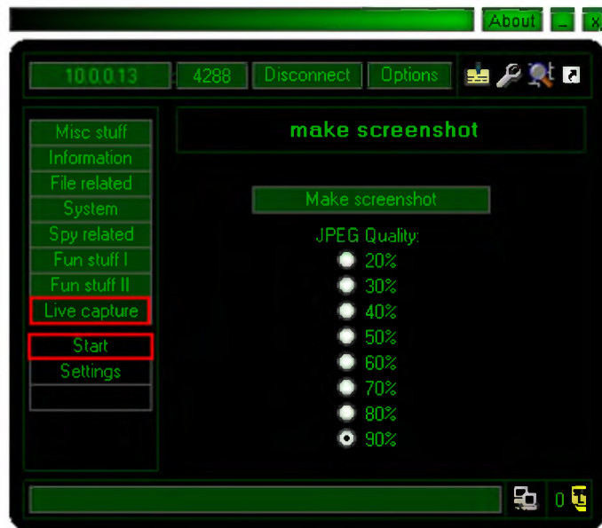
FIGURE 10.18: start capturing
