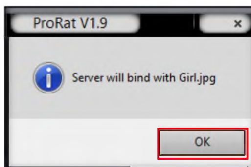
FIGURE 1.6: ProRat Pop-up
