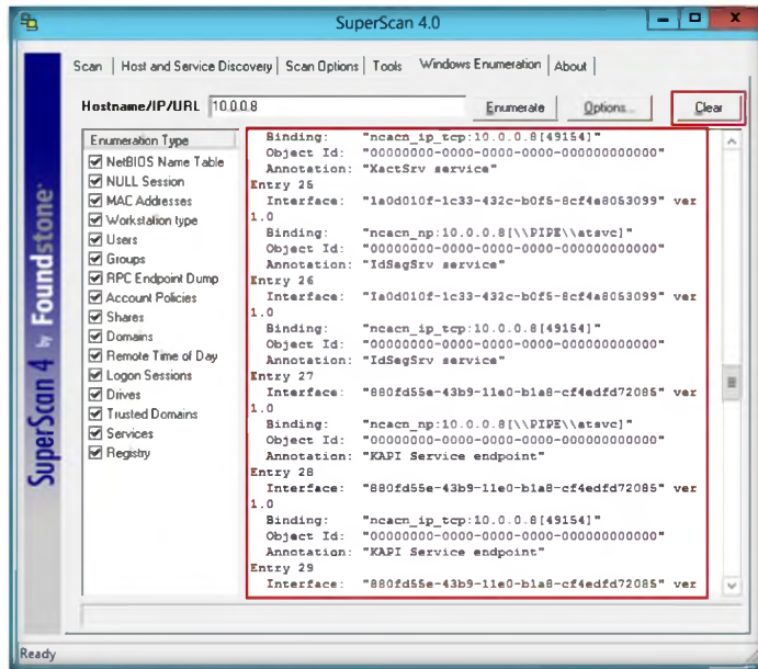
FIGURE 2.5: SuperScan main window with results
