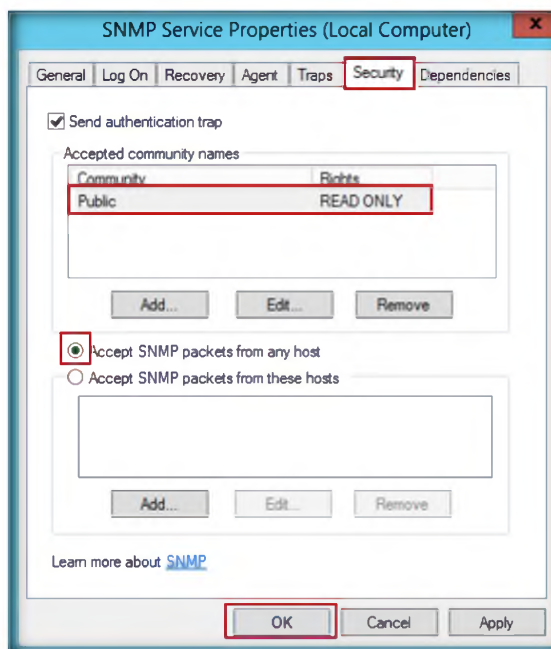
FIGURE 5.2: Configuring SNMP Services
