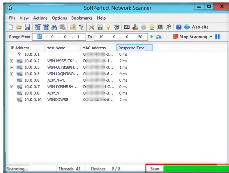
FIGURE 4.3: SoftPerfect status bar
