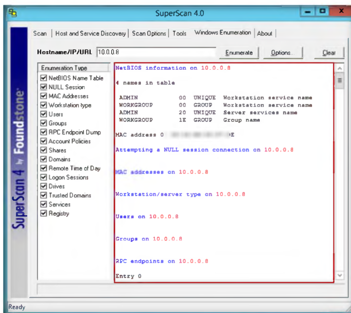
FIGURE 2.3: SuperScan main window with results
