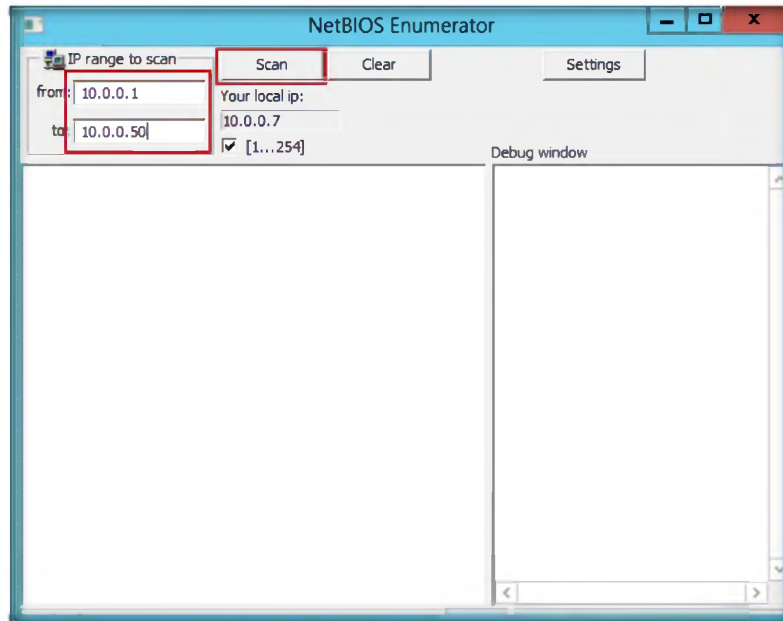
FIGURE 3.2: NetBIOS Enumerator with IP range to scan
