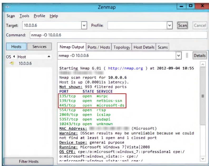
FIGURE 1.4: The Zenmap output window
