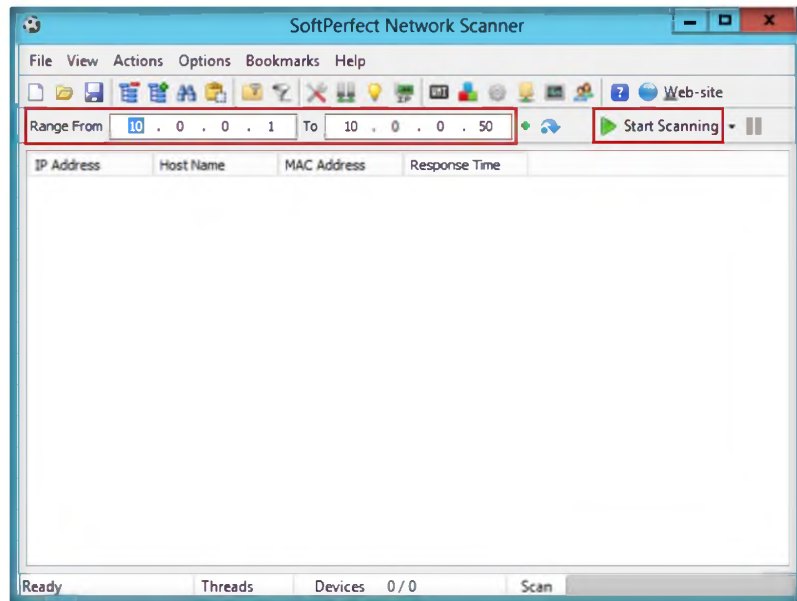
FIGURE 4.2: SoftPerfect setting an IP range to scan
