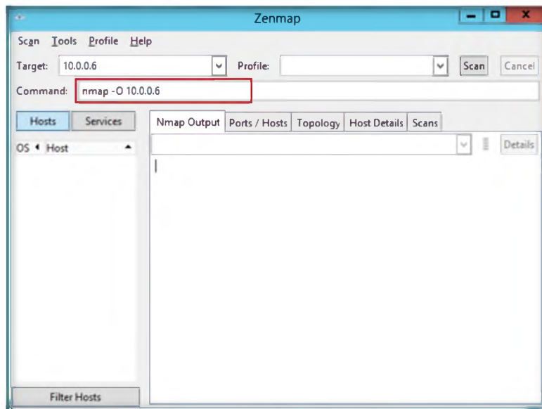
FIGURE 1.3: The Zenmap Main window
