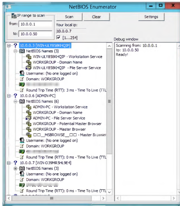
FIGURE 3.3: NetBIOS Enumerator results
