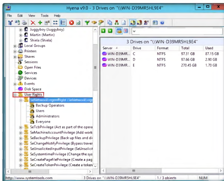
FIGURE 6.11: Users Rights
