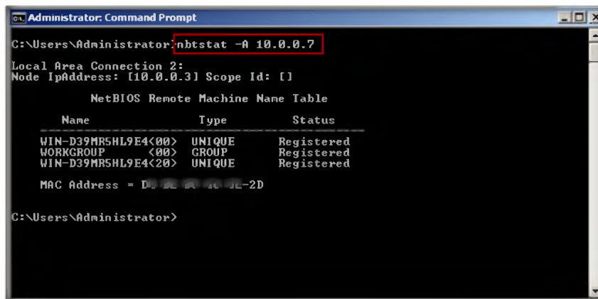
FIGURE 1.5: Command Prompt with the nbtstat command
