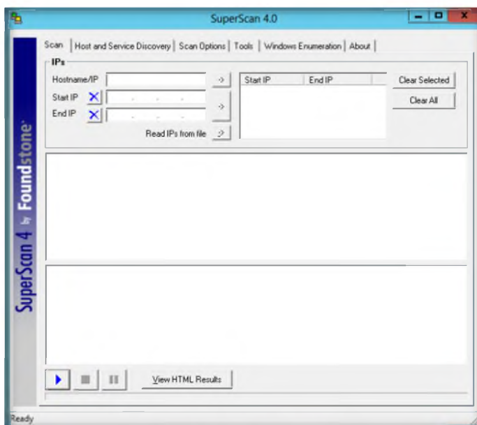
FIGURE 2.1: SuperScan main window
