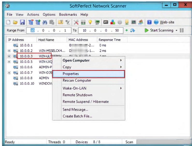
FIGURE 4.4: SoftPerfect IP address scanned details
