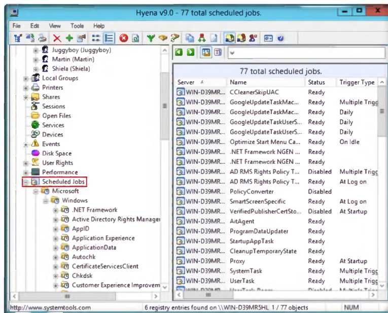
FIGURE 6.12: Scheduled jobs
